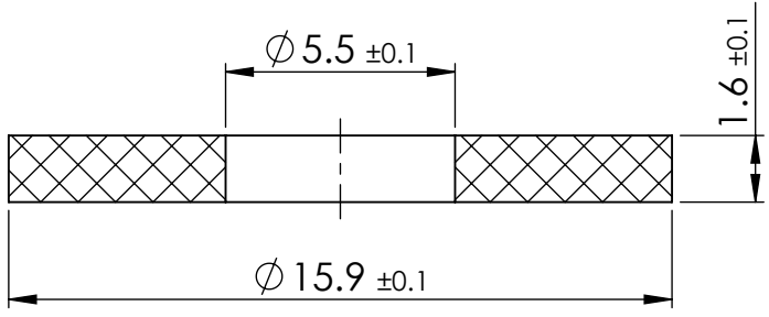
SECTION X-X
